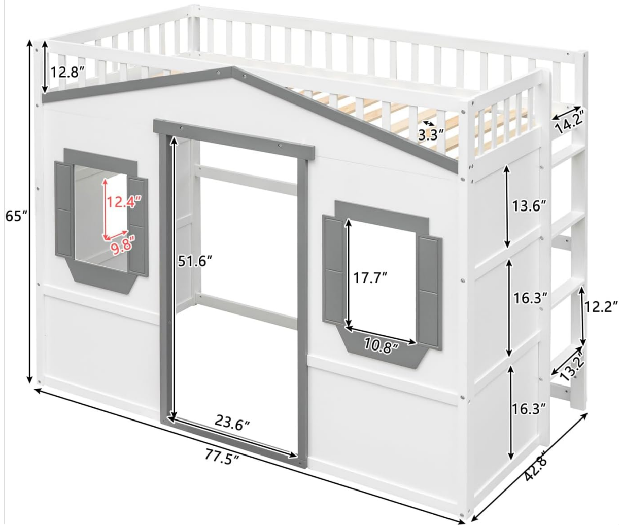
Image 7: A technical diagram illustrating the key dimensions of the TRIPLE TREE Twin Size House Loft Bed, including length, width, height, and specific measurements for the ladder and house structure components.
