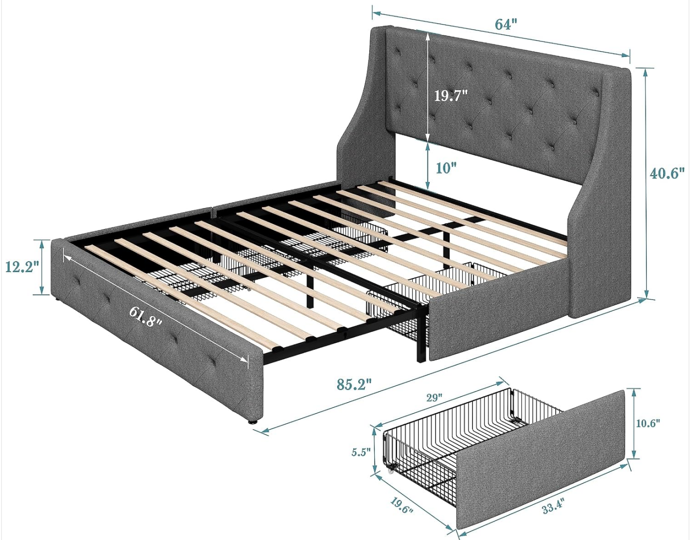
Image: Detailed diagram illustrating the dimensions of the Queen bed frame (85.2"L x 64"W x 40.6"H) and its components, including the headboard, frame, and storage drawers.
