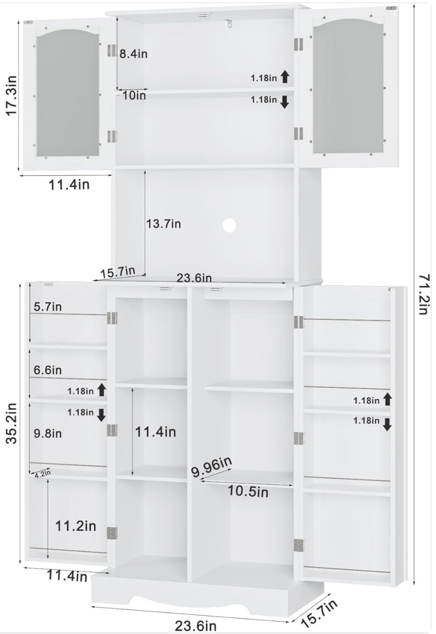
Figure 3.1: Product Dimensions and Weight Capacity Overview. This diagram illustrates the overall dimensions of the cabinet (15.7"D x 23.6"W x 71.2"H) and specifies the maximum weight capacities for the total unit (220 lbs), countertop (44 lbs), and upper shelves (22 lbs).
