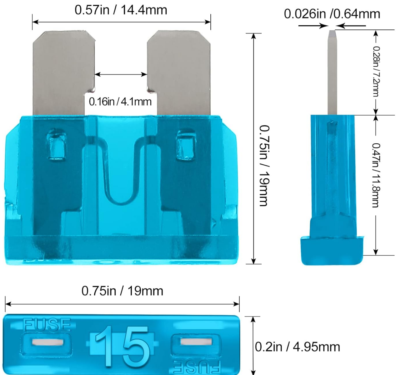
Figure 6.1: Dimensional specifications of a standard JOREST fuse.
