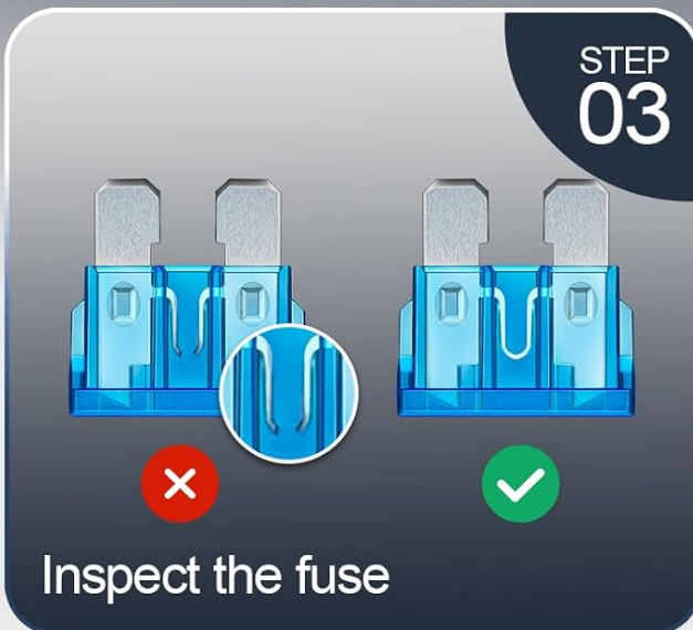
Figure 2.1: Step-by-step visual instructions for replacing a vehicle fuse.
