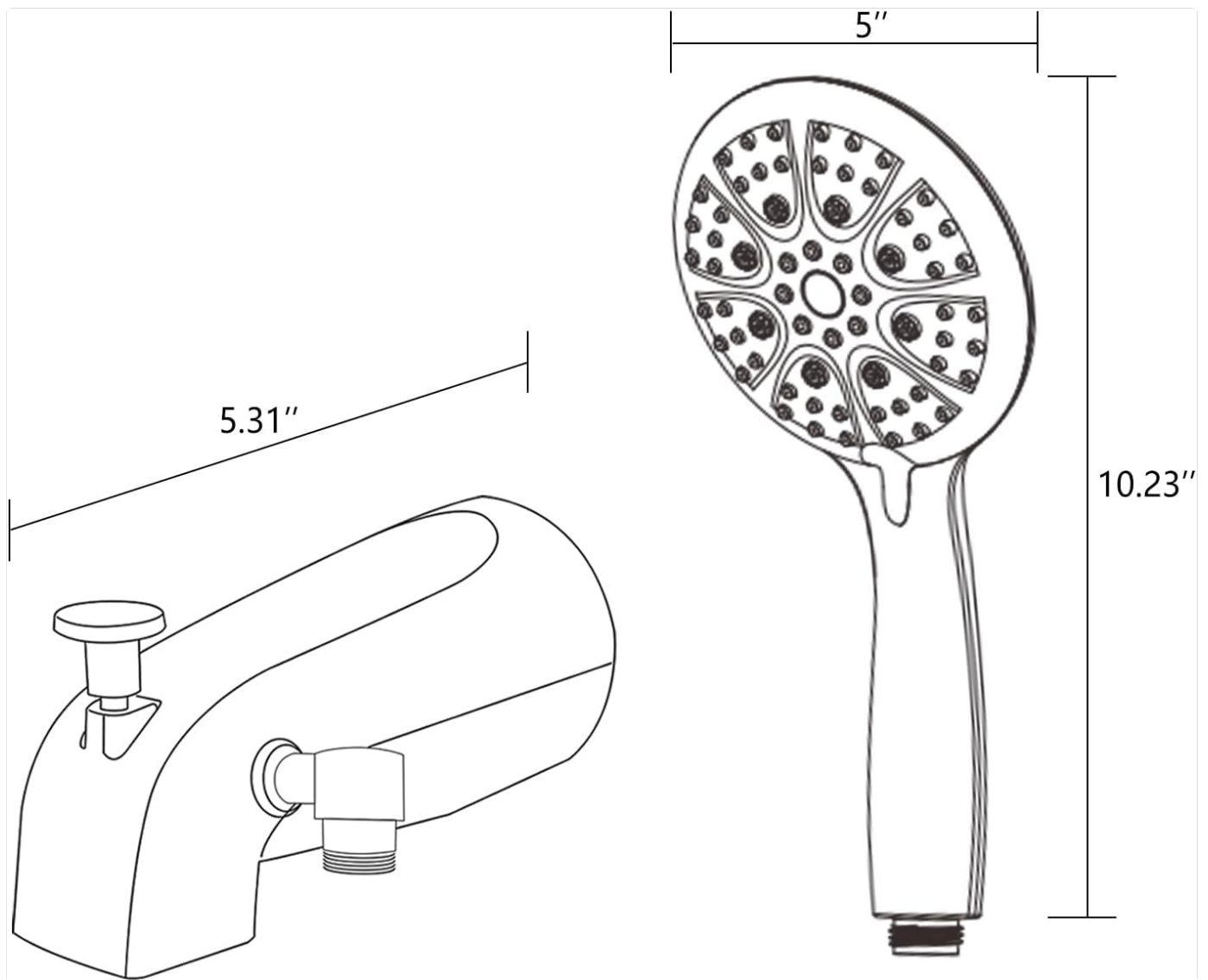
Figure 4: Product dimensions for planning installation.
