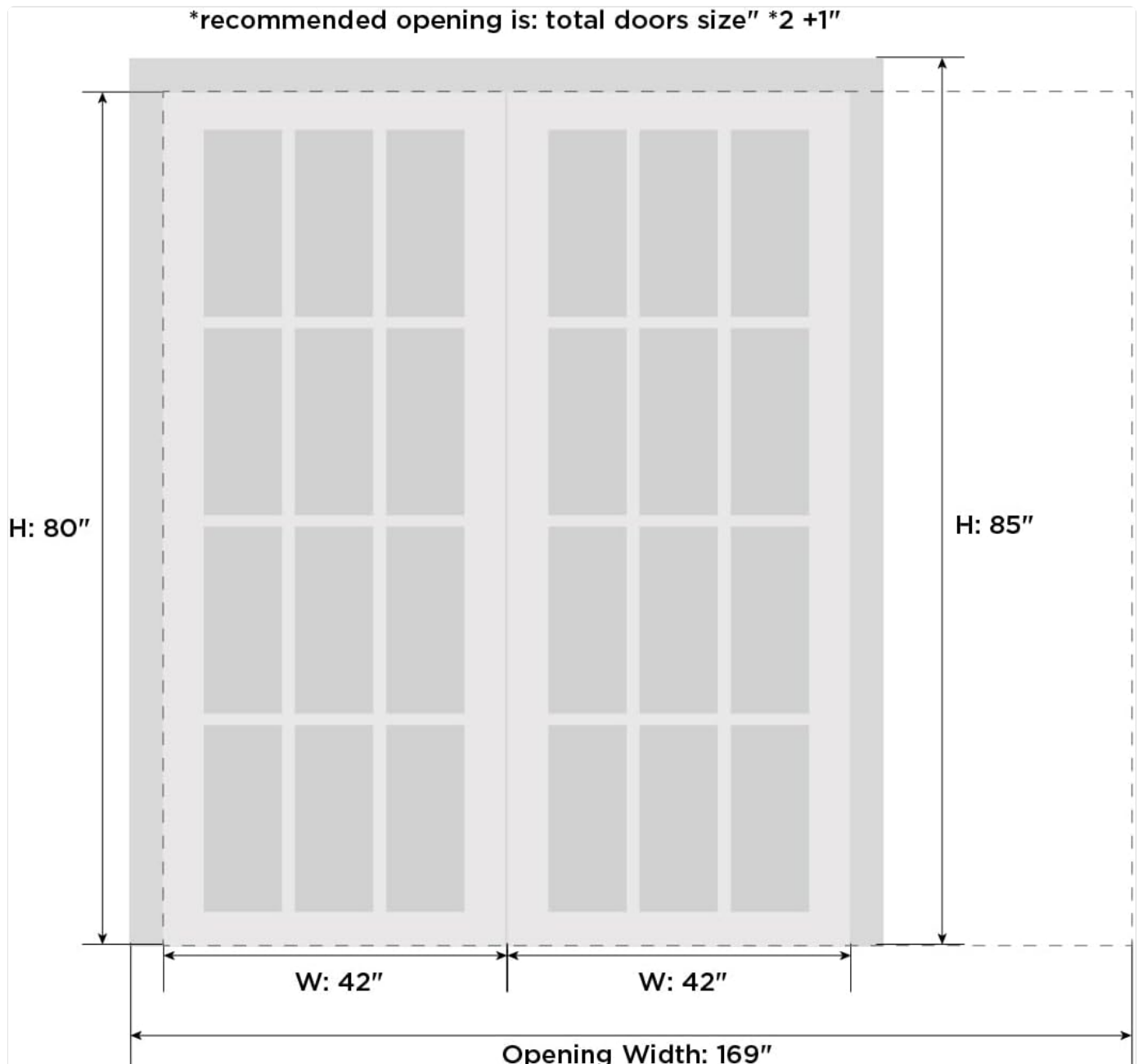
Figure 2: Diagram illustrating recommended opening dimensions for double pocket doors. The diagram shows the recommended height (H: 85") and total opening width (169") for two 42" x 80" door slabs.
