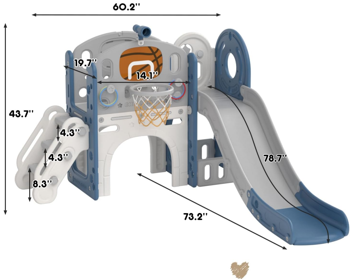
Image 8.1: Detailed dimensions of the assembled playset.
