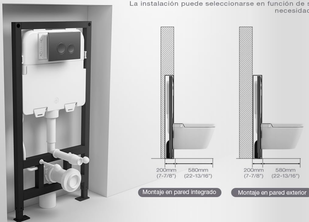
Figure 5: Depicts two mounting options: integrated wall mounting (flush with the wall) and exterior wall mounting (slightly protruding or for specific wall constructions). Dimensions for both are provided.
