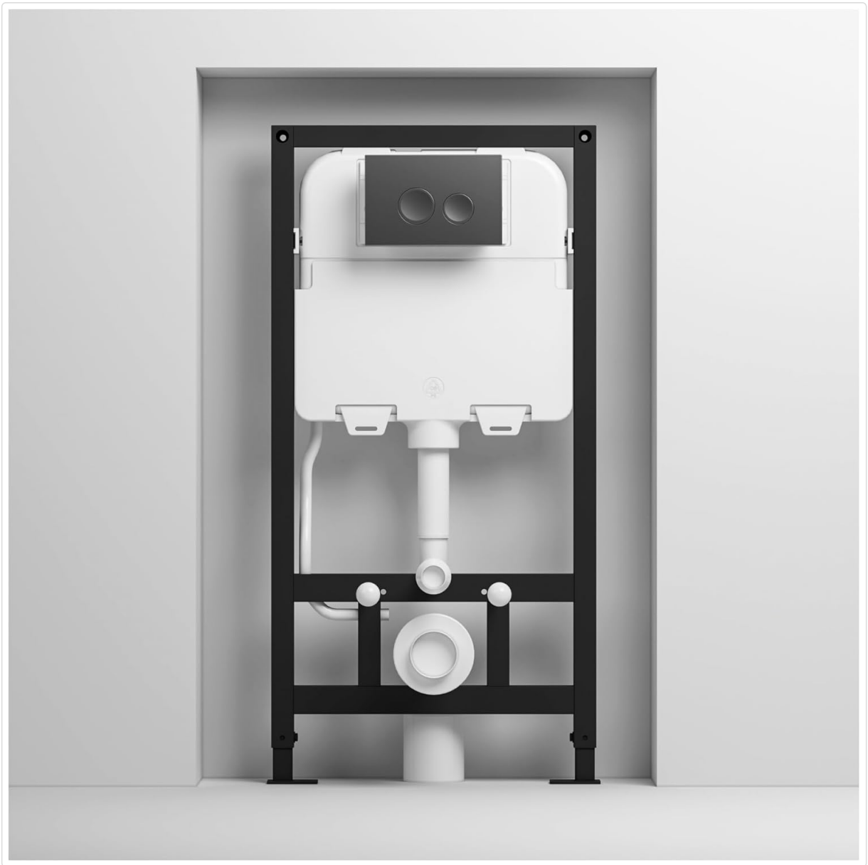
Figure 1: MEJE MZE014P In-Wall Flush Tank and Support System, showing the metal frame, concealed cistern, and flush plate mechanism.
