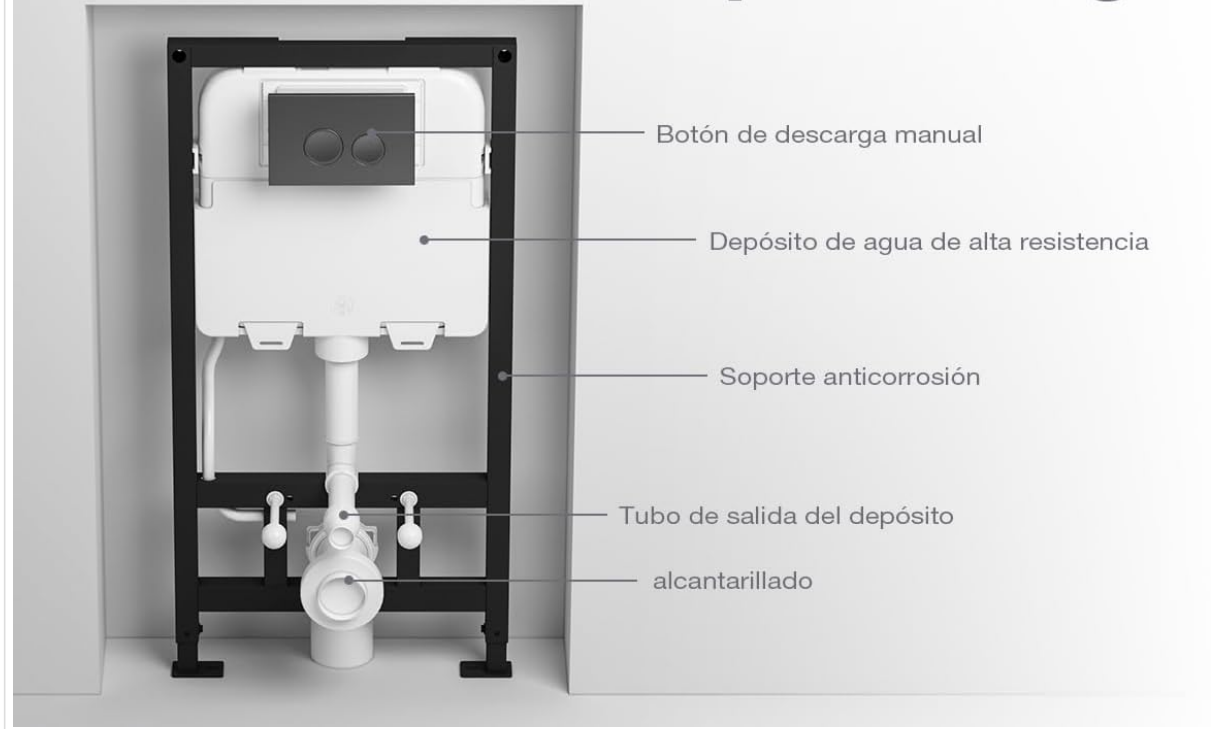
Figure 4: Labeled diagram of the in-wall flush tank system components, including the manual flush button, high-resistance water tank, anti-corrosion support, tank outlet pipe, and sewage connection.
