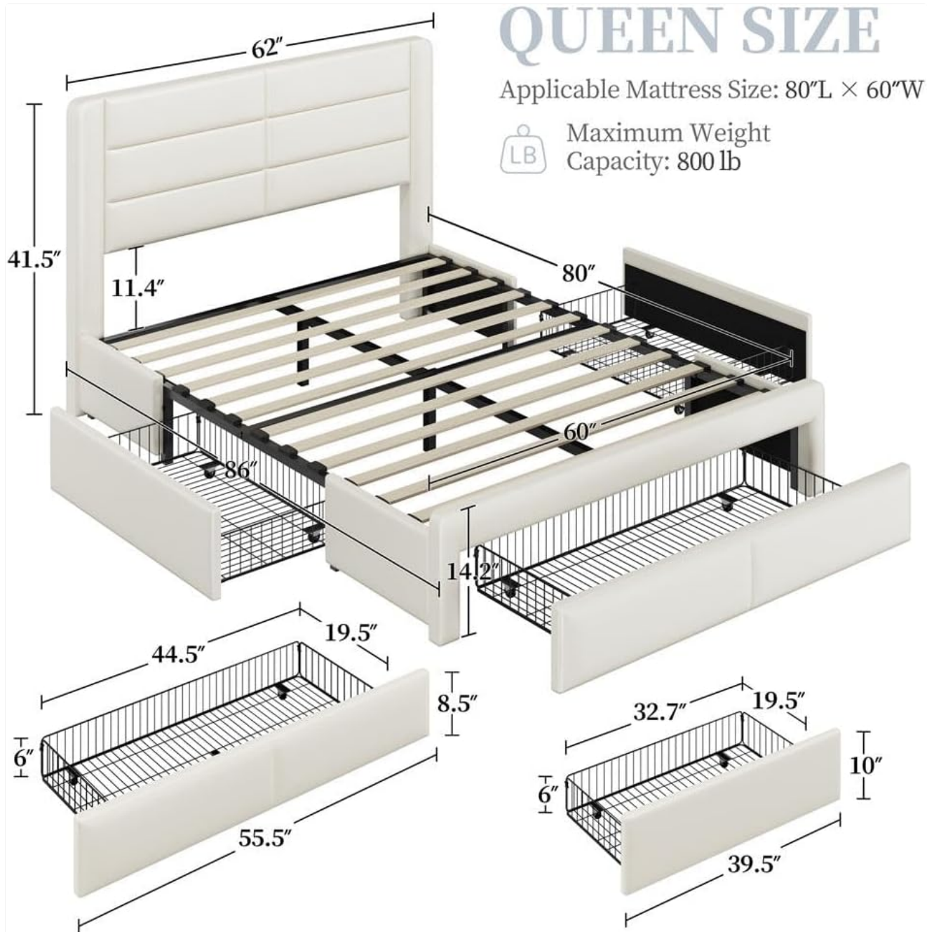
Image: Overall dimensions and key features of the Yaheetech Queen Size Bed Frame. The diagram shows the headboard height (41.5"), bed length (86"), bed width (62"), and drawer dimensions.
