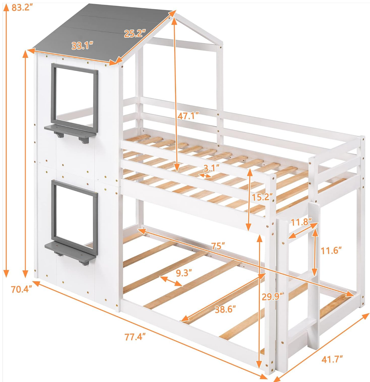
Image: A technical diagram illustrating the precise measurements of the Bellemave Twin Over Twin House Bunk Bed. Key dimensions shown include overall length (77.4"), width (41.7"), and height (83.2"), as well as internal bunk dimensions, ladder height, and roof angles.
