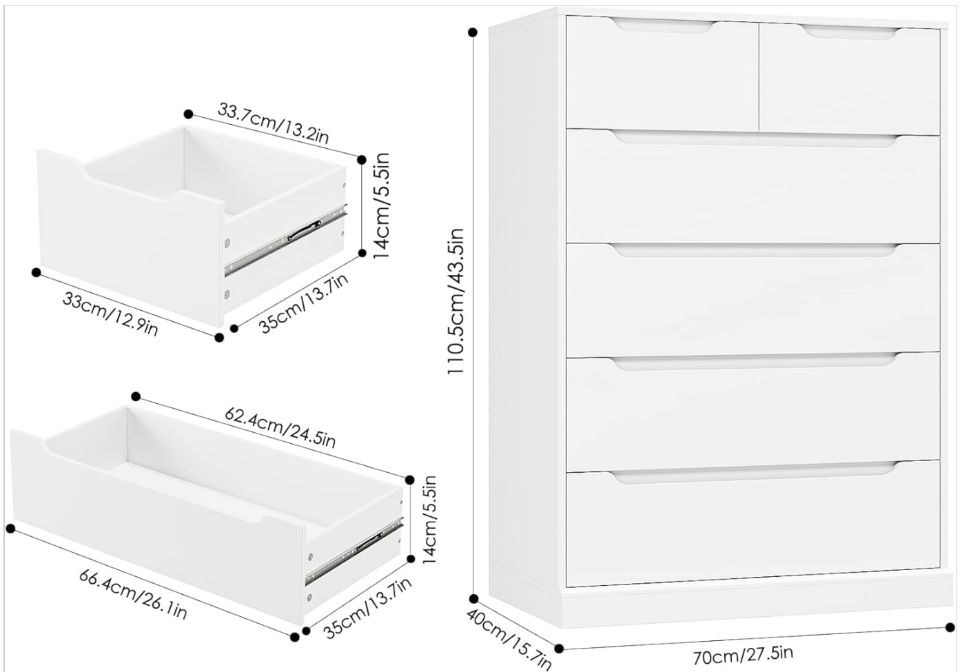
Image: Diagram showing the overall dimensions of the dresser (110.5cm/43.5in height, 70cm/27.5in width, 40cm/15.7in depth) and the internal dimensions of the two types of drawers.
