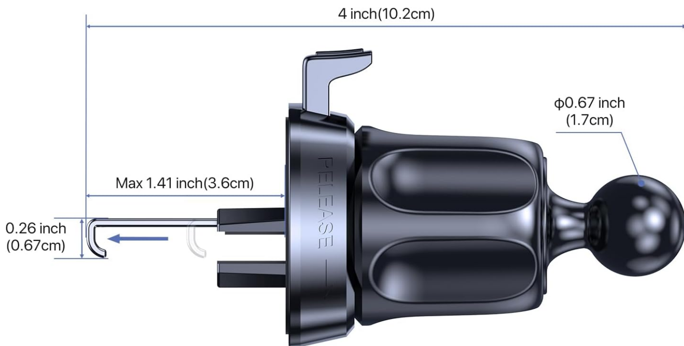
Figure 5: Dimensions of the air vent clip for compatibility reference.
