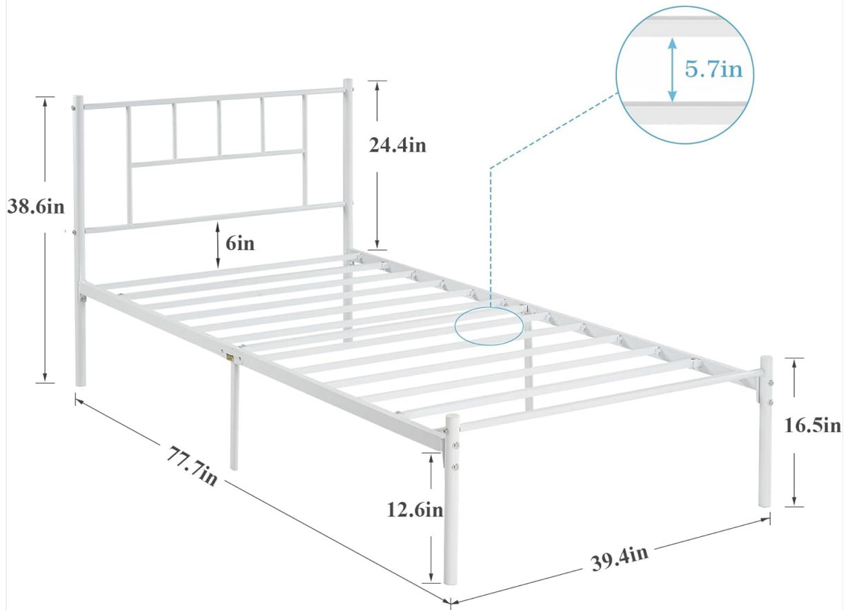
Figure 6: Detailed dimensional drawing of the VECELO Twin Metal Platform Bed Frame, including length, width, height, and under-bed clearance measurements.
