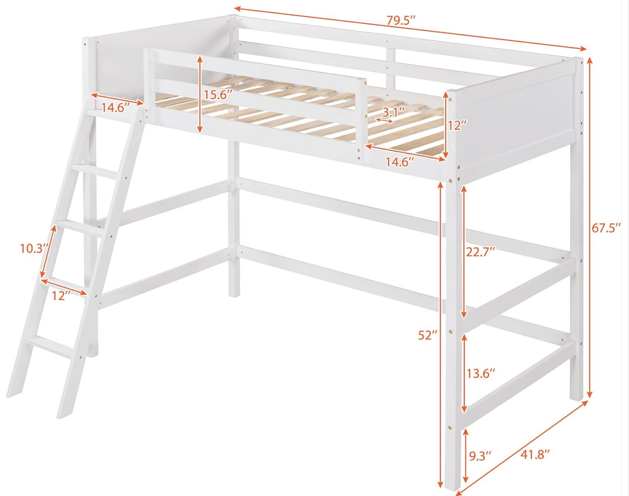
Figure 4.2: Dimensional diagram of the loft bed, indicating key measurements.
