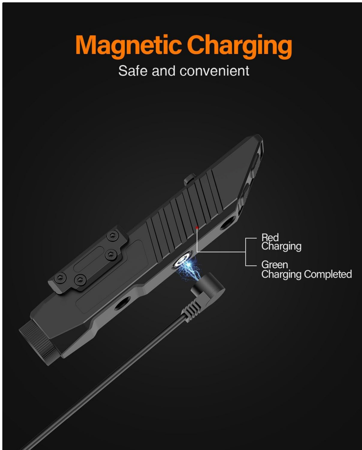
Figure 5: Magnetic charging in progress (red indicator) and charging completed (green indicator).
