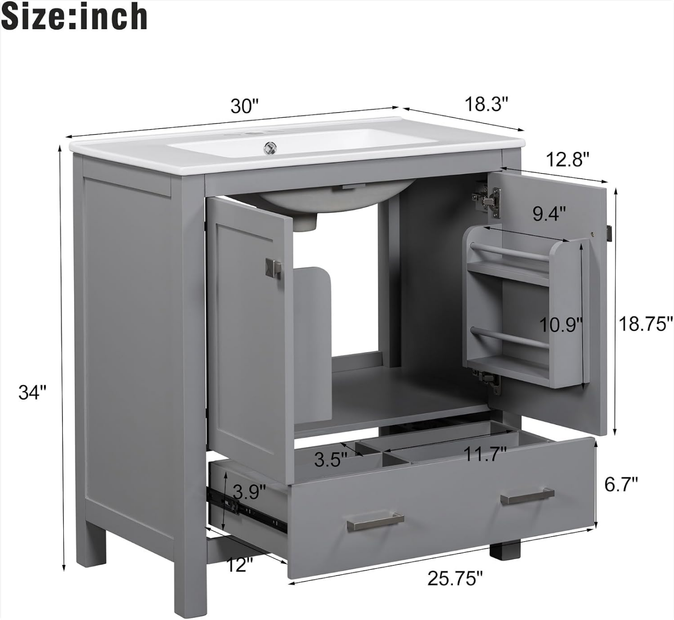
Image: Technical drawing of the vanity with precise measurements for overall dimensions, door size, and drawer dimensions.
