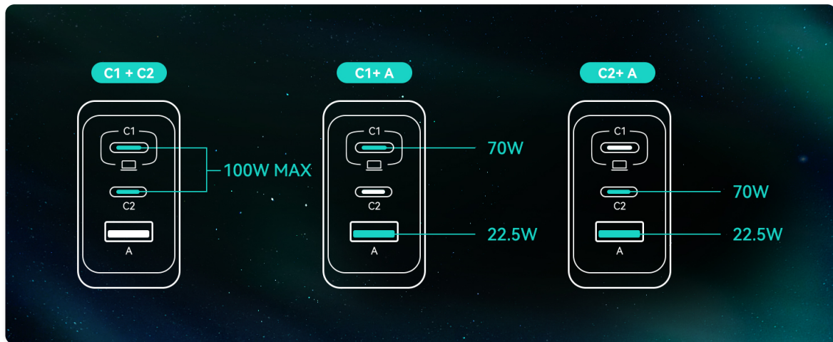
Figure 6: Individual port power output.
