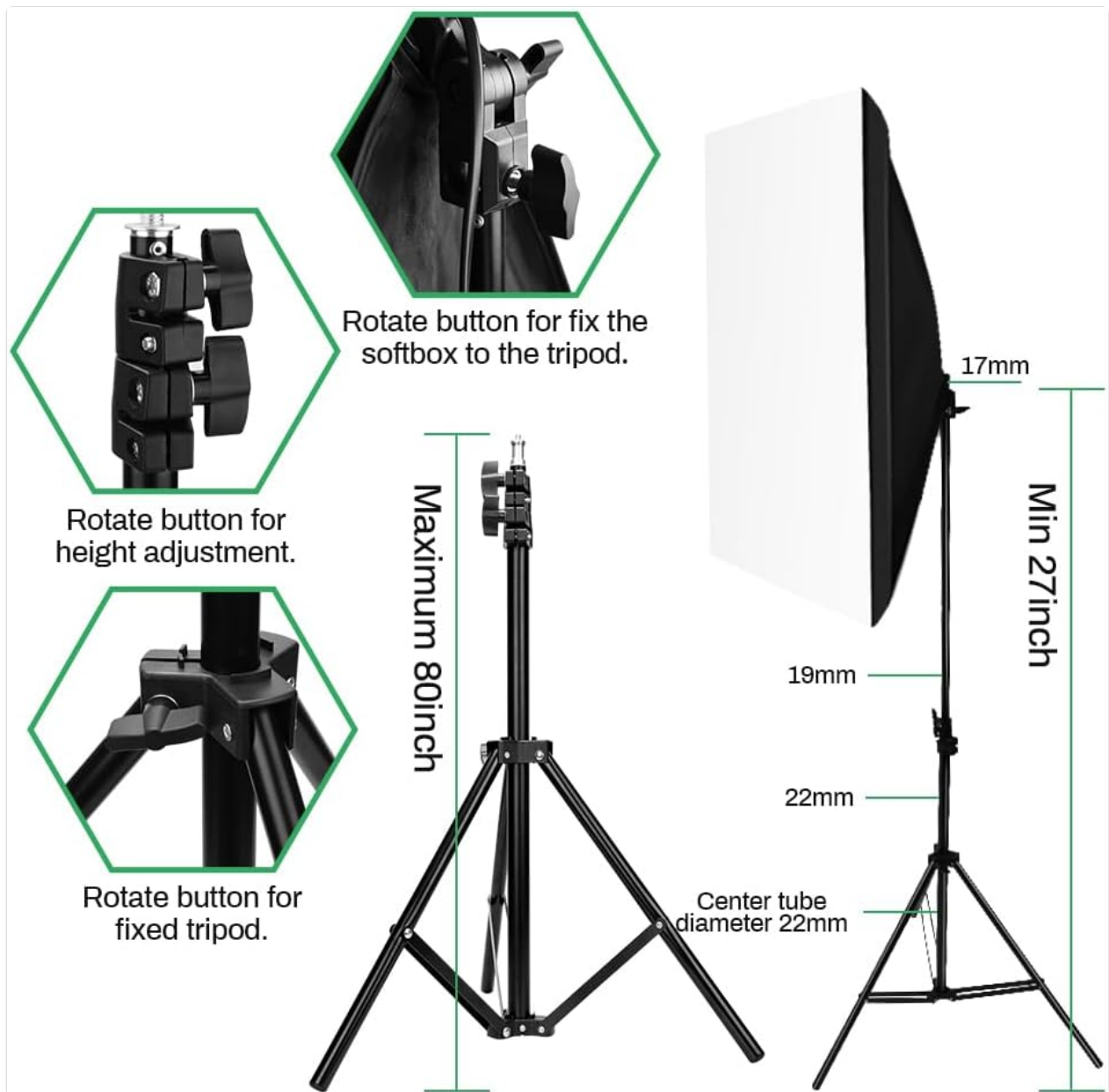
Image: Detailed view of the tripod stand, highlighting the rotation buttons for fixing the softbox, adjusting height, and securing the tripod legs.
