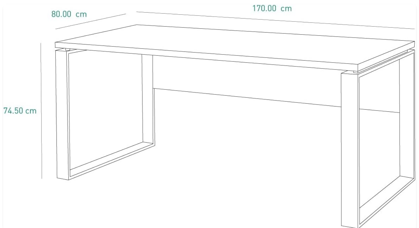
Image 3.2: Dimensional diagram of the Composad DISEGNO desk, showing width (170 cm), depth (80 cm), and height (74.5 cm).
