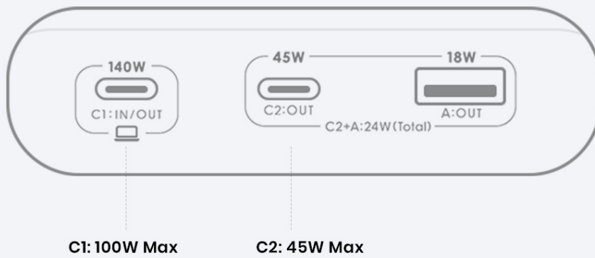
Image: Diagram showing power output for two-port charging (C1 + A).
