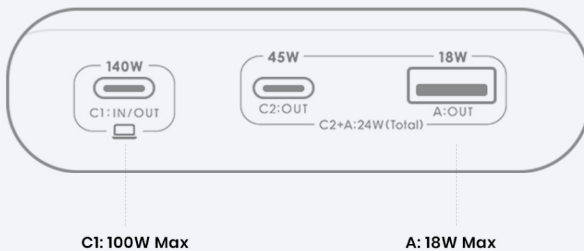
Image: Diagram showing power output for three-port charging (C1 + C2 + A).
