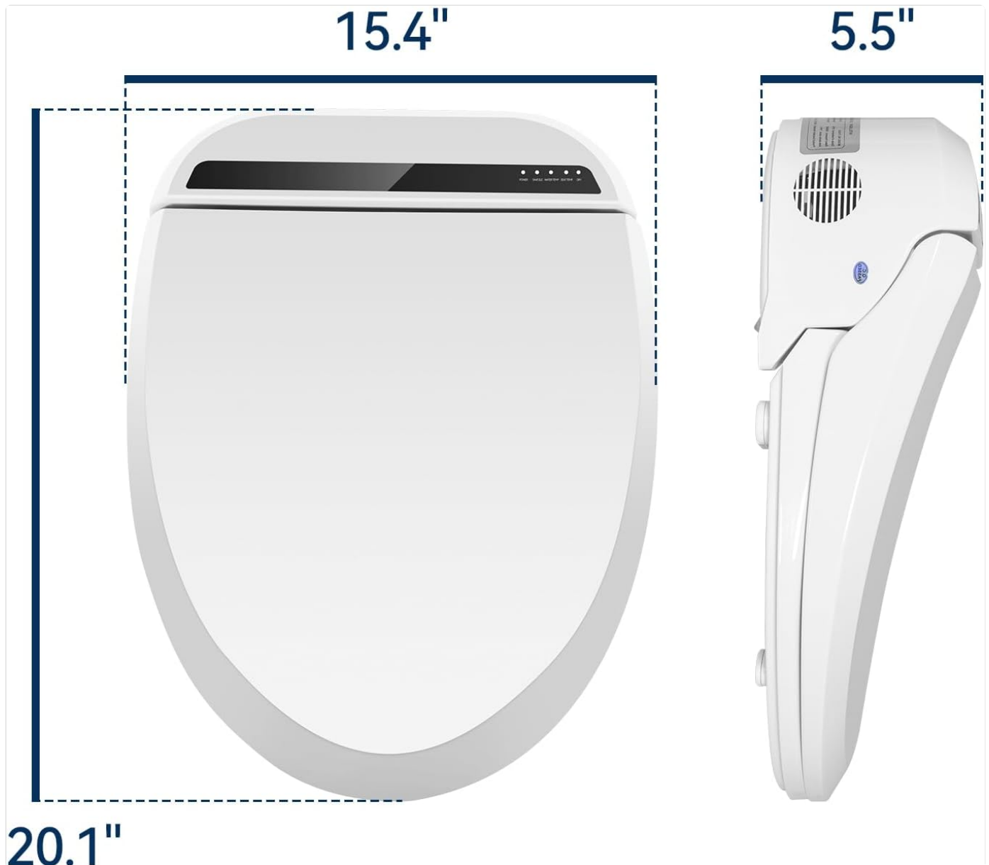
Image: Top and side view of the bidet toilet seat showing its dimensions: 20.1 inches in length and 15.4 inches in width. The side profile shows a height of 5.5 inches.
