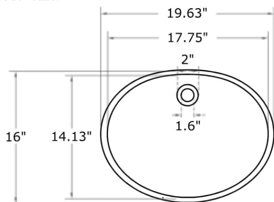
Image 3.1: Detailed dimensions diagram for the ARIEL Oval Undermount Sink.
