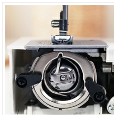
Figure 4: View of the bobbin area for insertion.
