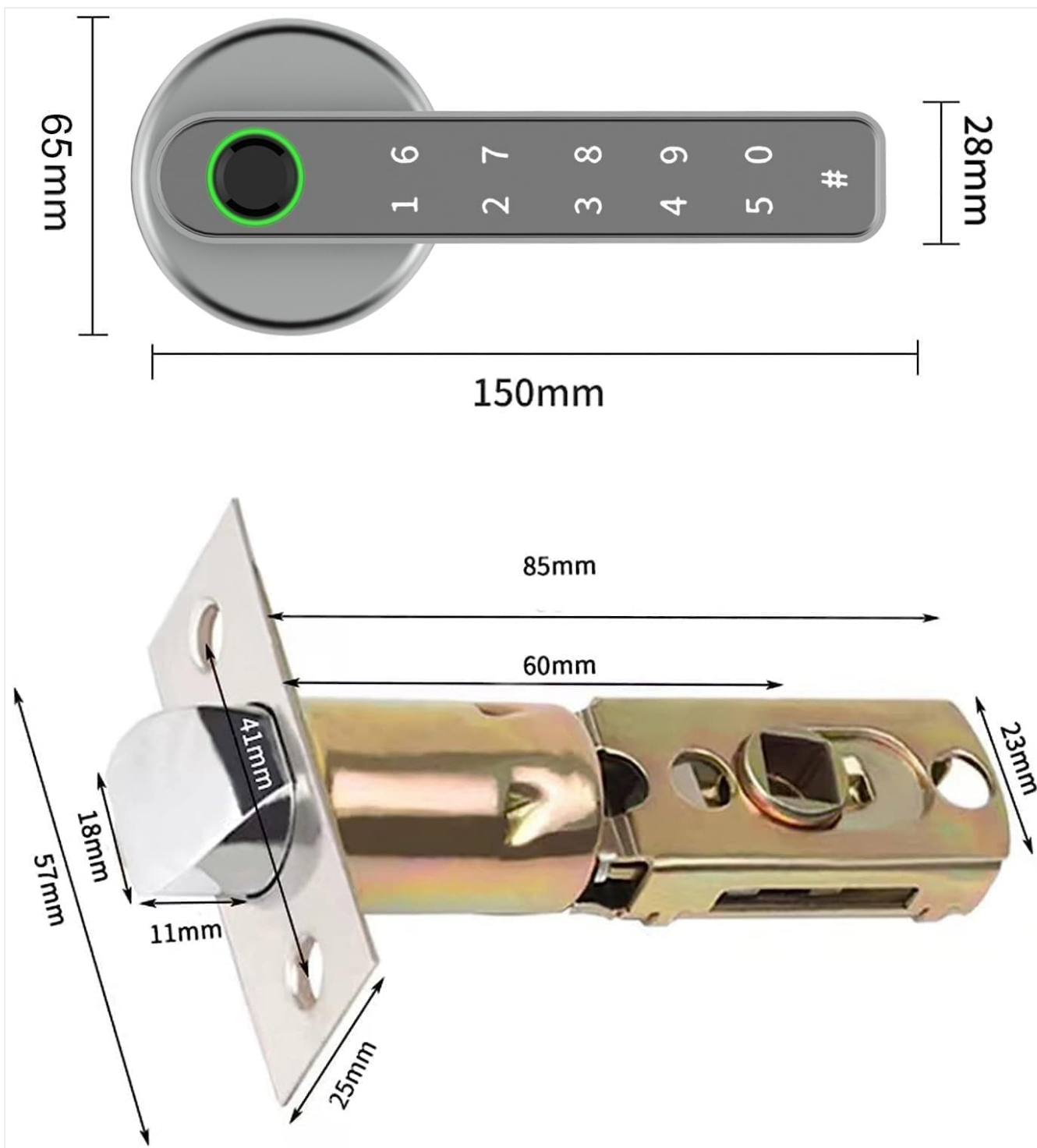
Image: Technical dimensions of the smart lock handle (150mm length, 65mm height, 28mm width) and the latch bolt (85mm length, 60mm backset, 57mm height).
