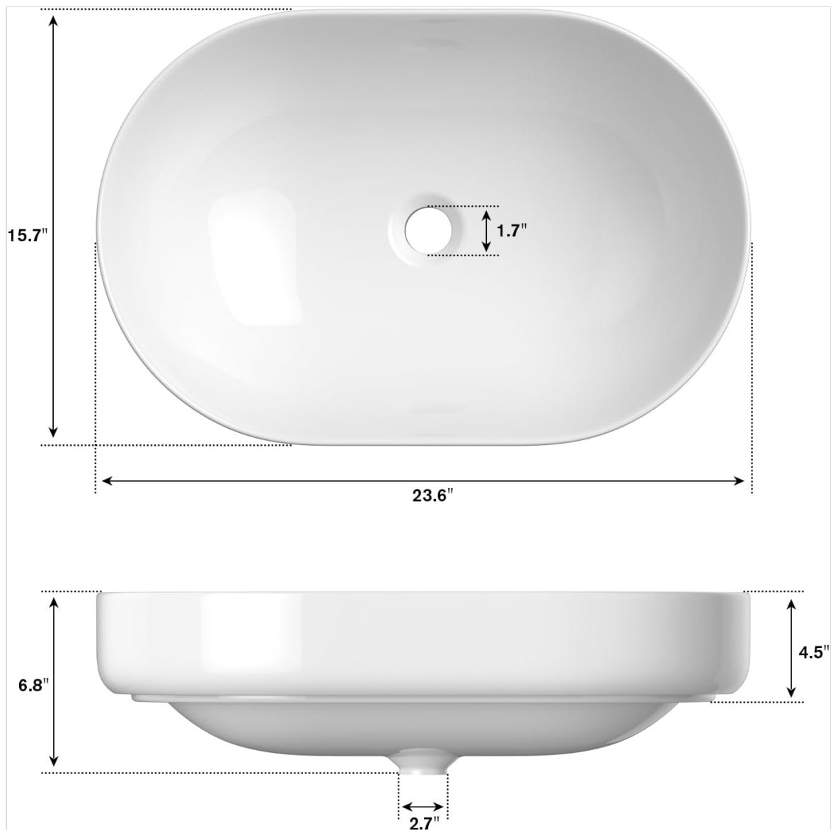
Image: Detailed dimensions diagram for the vessel sink.
