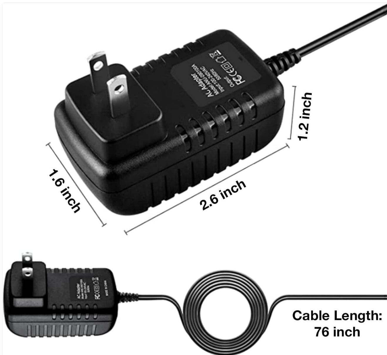
Image 3.2: Dimensions of the adapter (1.6 inches x 2.6 inches x 1.2 inches) and cable length (76 inches). These measurements ensure a compact design with adequate reach.
