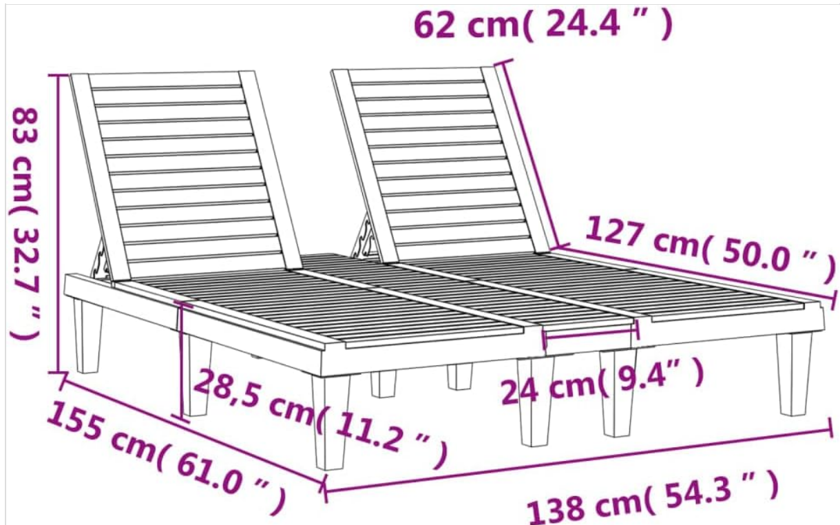
Image 4.1: Dimensional overview of the sun lounger. Overall dimensions are approximately 61.0" (155 cm) W x 54.3" (138 cm) D x 32.7" (83 cm) H.
