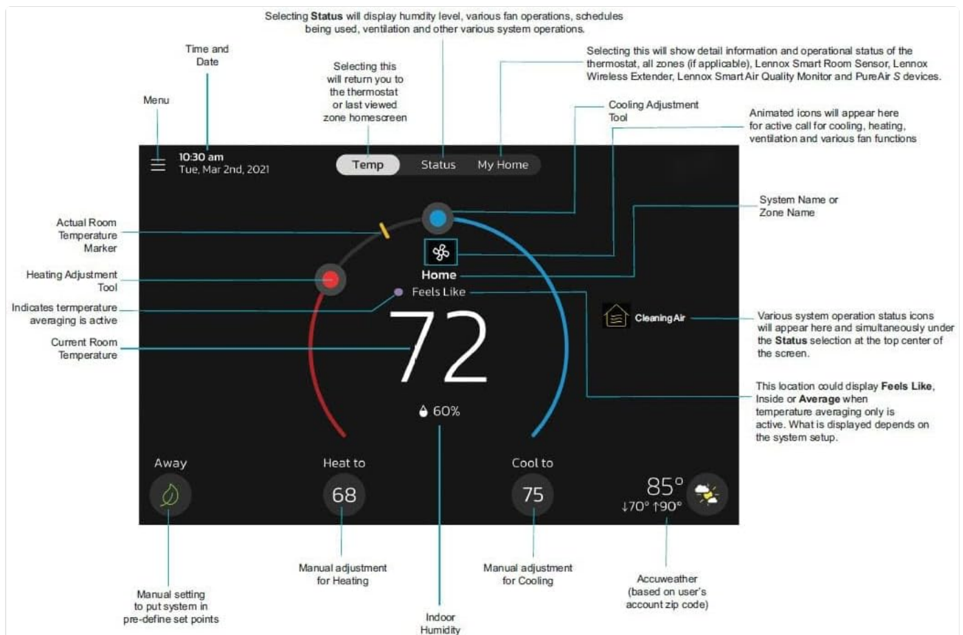
Figure 3: Annotated Lennox S40 Thermostat Display
