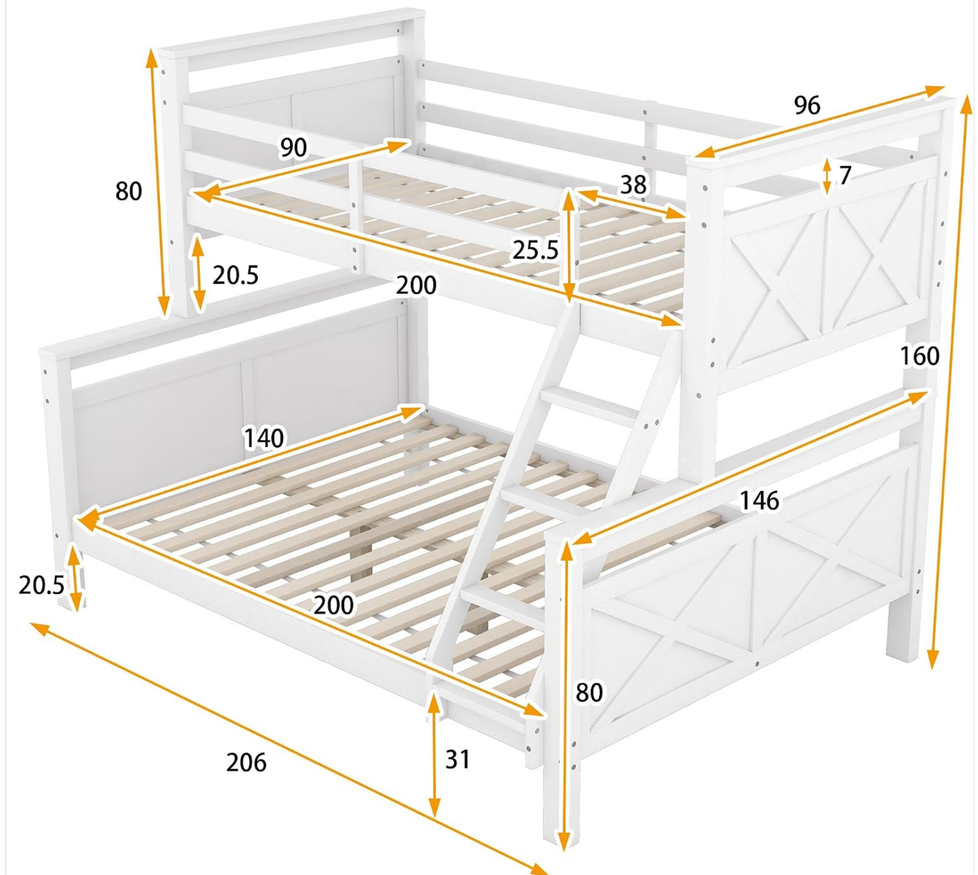
Figure 2: Detailed dimensions of the Moimhear Bunk Bed in centimeters. The diagram illustrates the length, width, and height of both the upper and lower bunks, as well as the overall structure.
