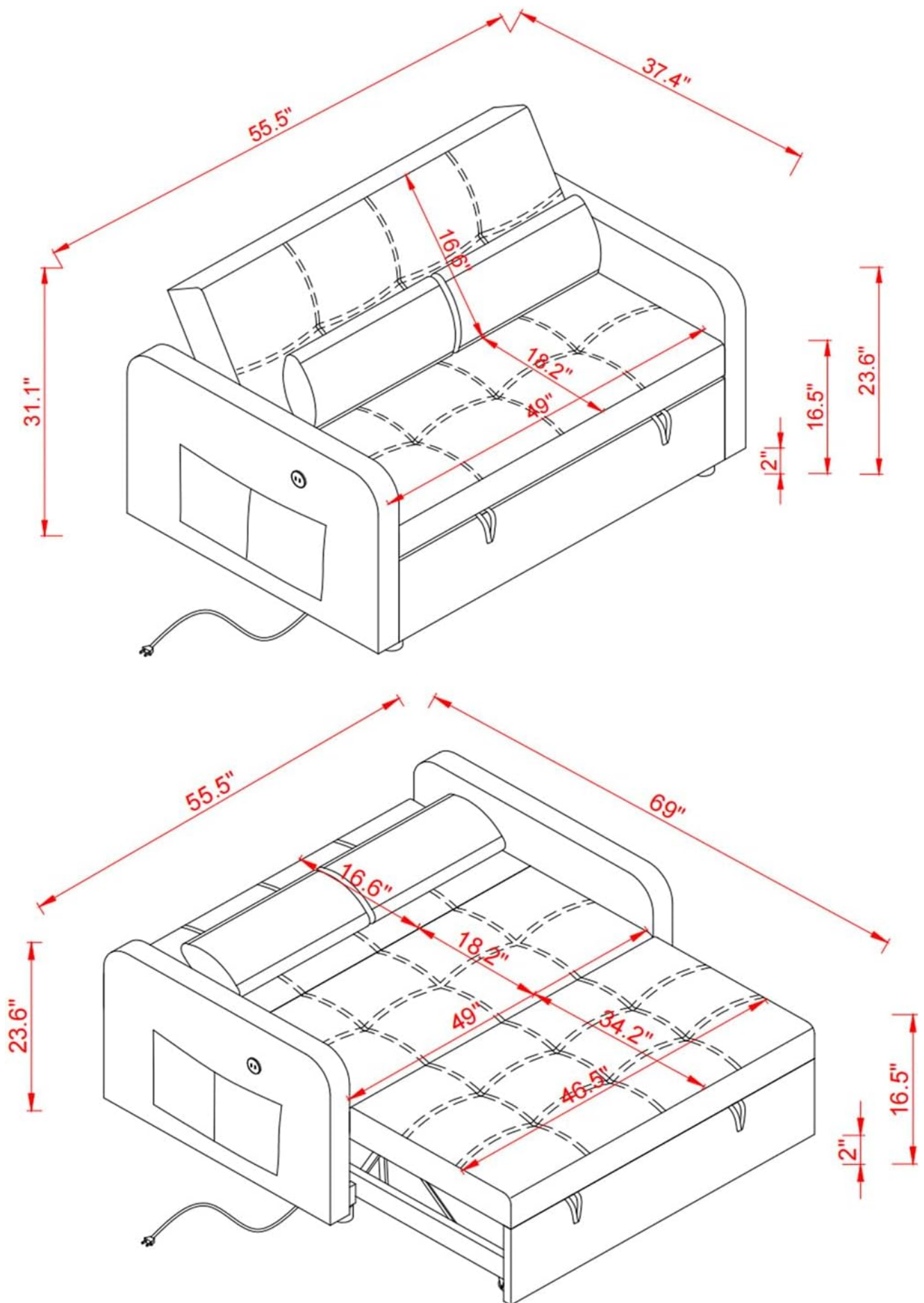
Image: Detailed dimension diagram for the sofa bed in both its compact (sofa) and extended (bed) forms.
