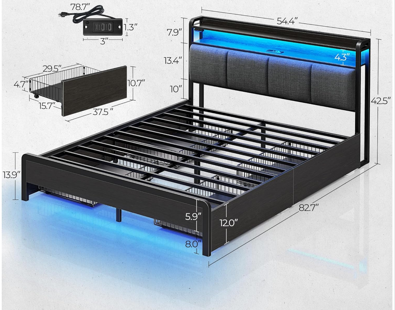
Figure 1: Overview of all bed frame components.
