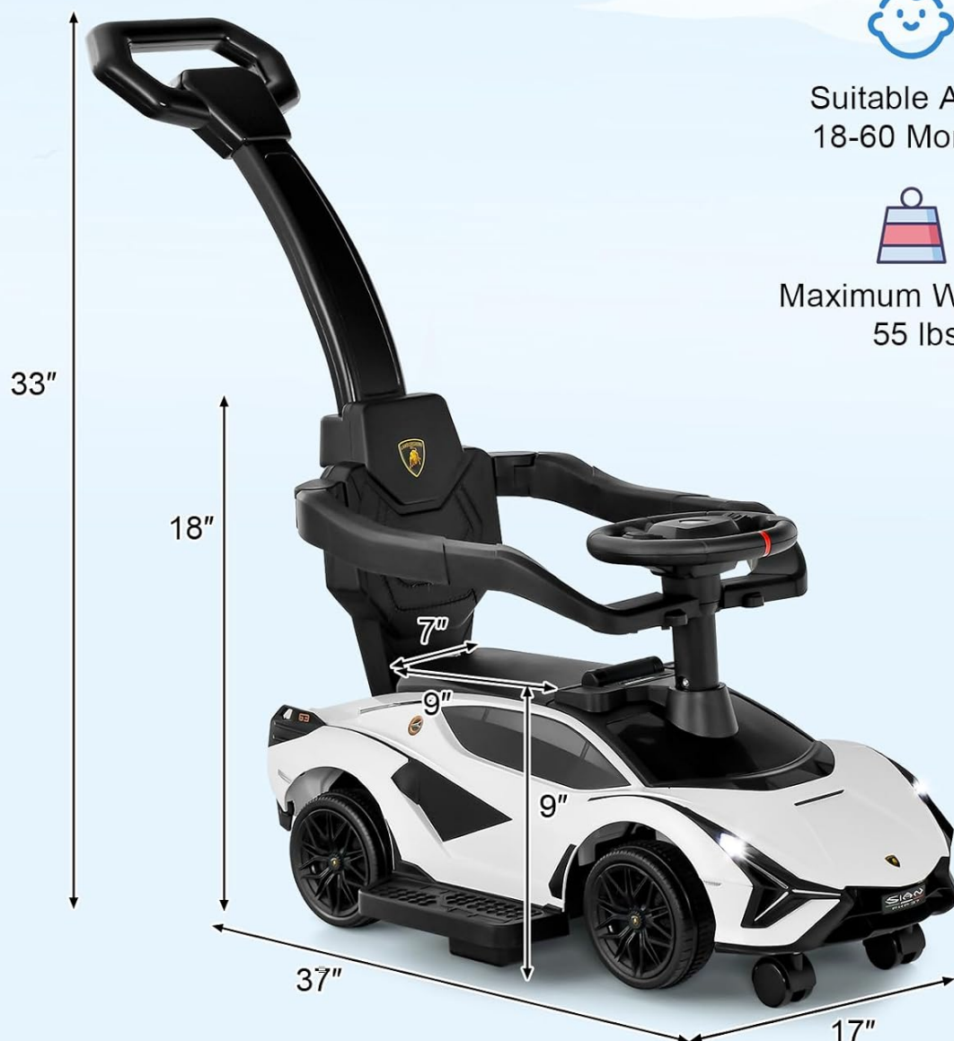
Figure 8: Product Dimensions.
