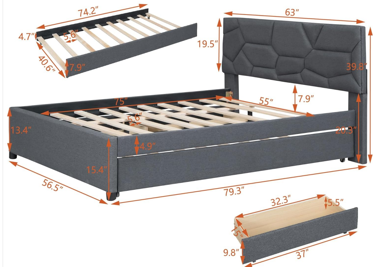
Figure 7: Product dimensions.
