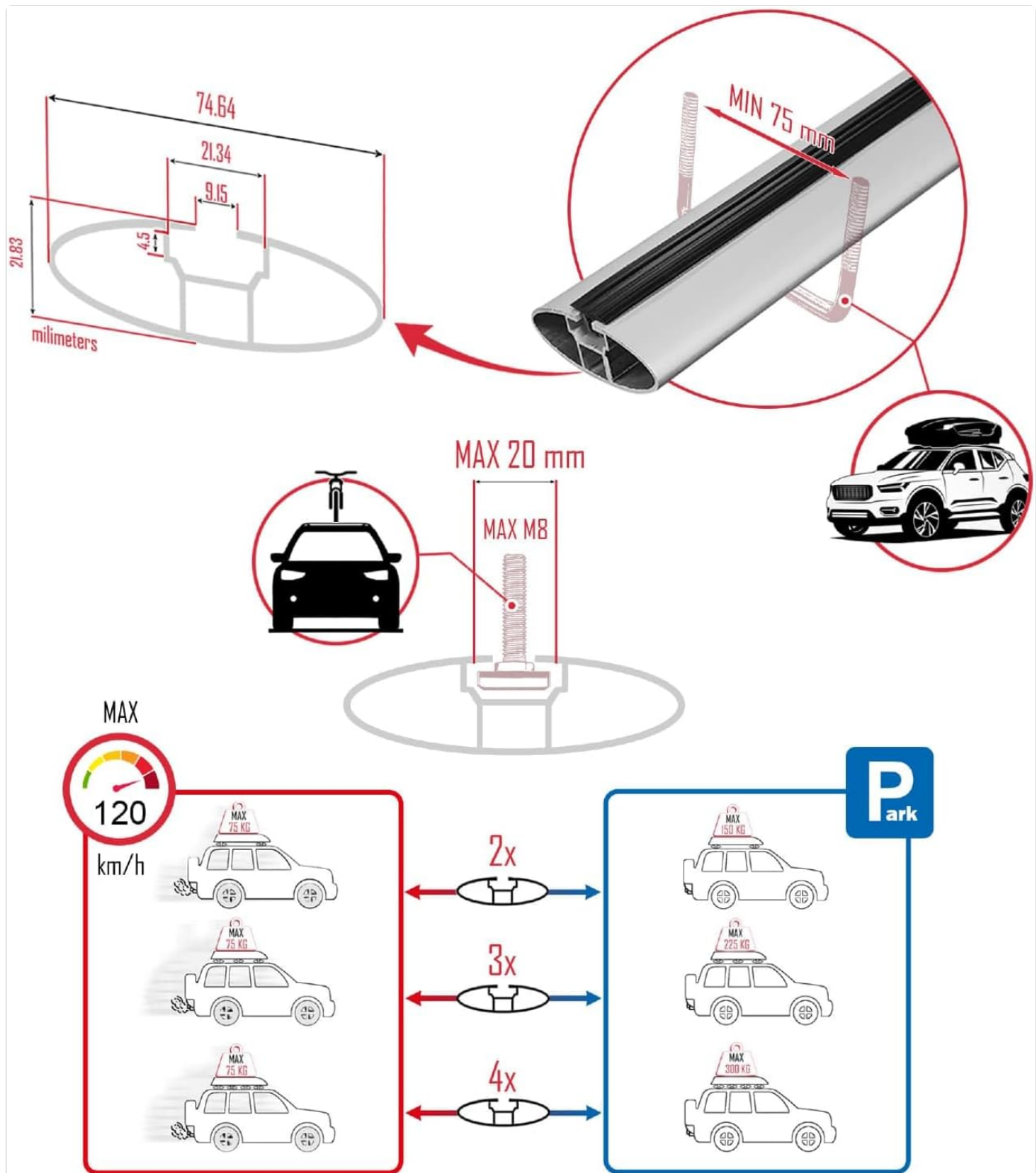
Image: Load capacity guidelines for moving and parked vehicles.
