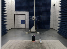
RADIATED EMISSION TEST SETUP ABOVE 1GHZ
