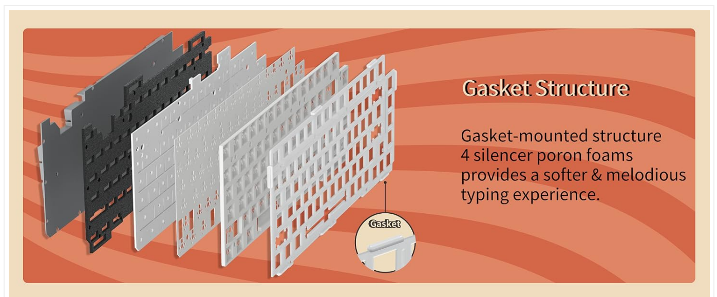
Image: Exploded view illustrating the gasket mount structure with multiple sound-dampening layers for enhanced typing feel and acoustics.
