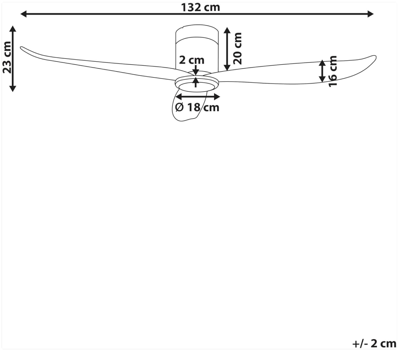
Image: A technical diagram illustrating the dimensions of the Beliani Malad Ceiling Fan. Key measurements include a total width of 132 cm, a height of 23 cm, and a base diameter of 18 cm.
