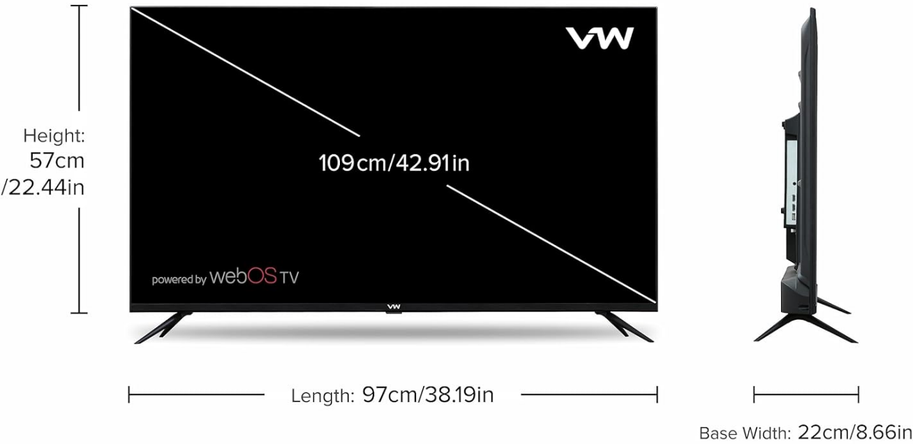
Image: Diagram showing the dimensions of the VW QLED TV, including height (57cm/22.44in), length (97cm/38.19in), and base width (22cm/8.66in), with a diagonal screen size of 109cm/42.91in.
