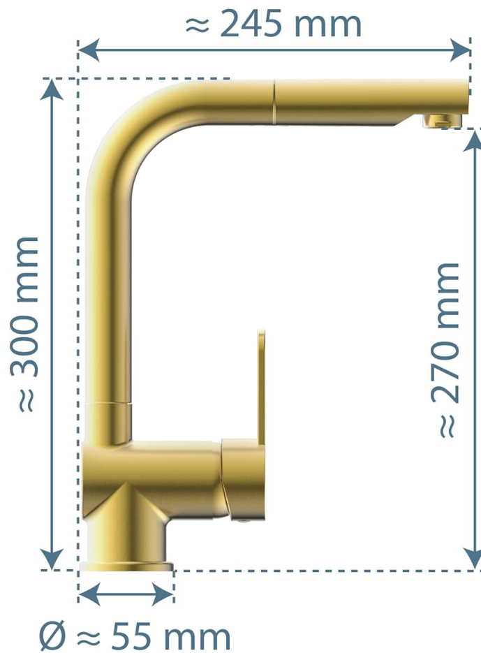
Image 8.1: Detailed technical dimensions of the SCHÜTTE London 79770 faucet.
