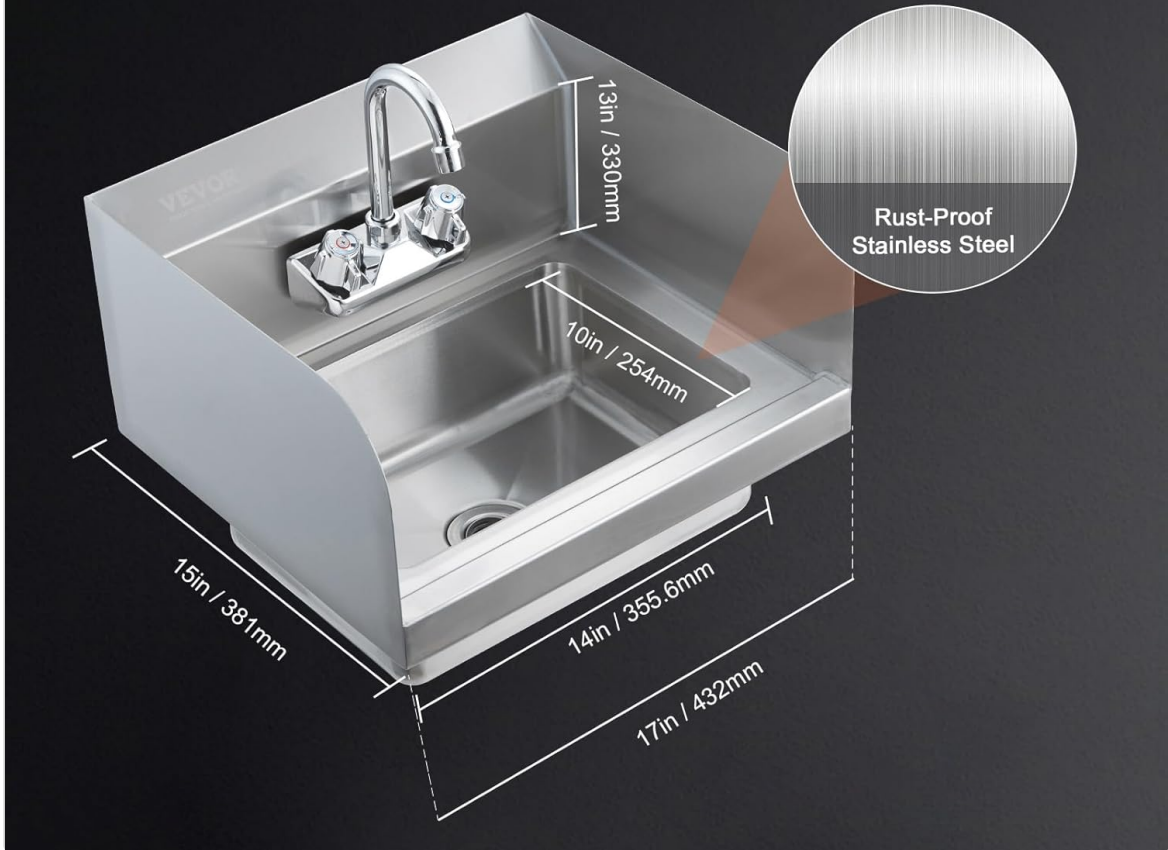
Image 6.1: Key dimensions of the VEVOR Commercial Hand Sink.
