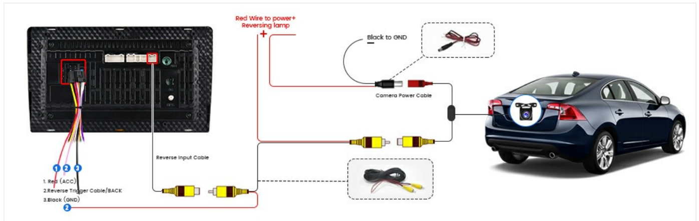
Image: Diagram illustrating the connection of the AHD backup camera to the car stereo and the vehicle's reverse light circuit.
