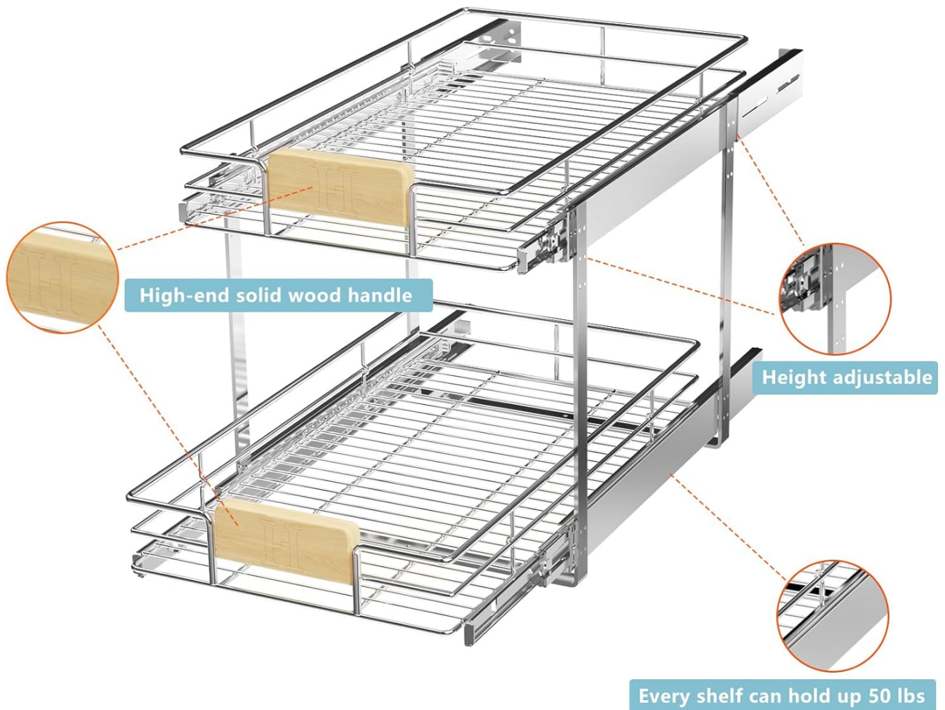
Image: Detailed view of the assembled pull-out organizer, highlighting the wooden handles and height adjustment points.
