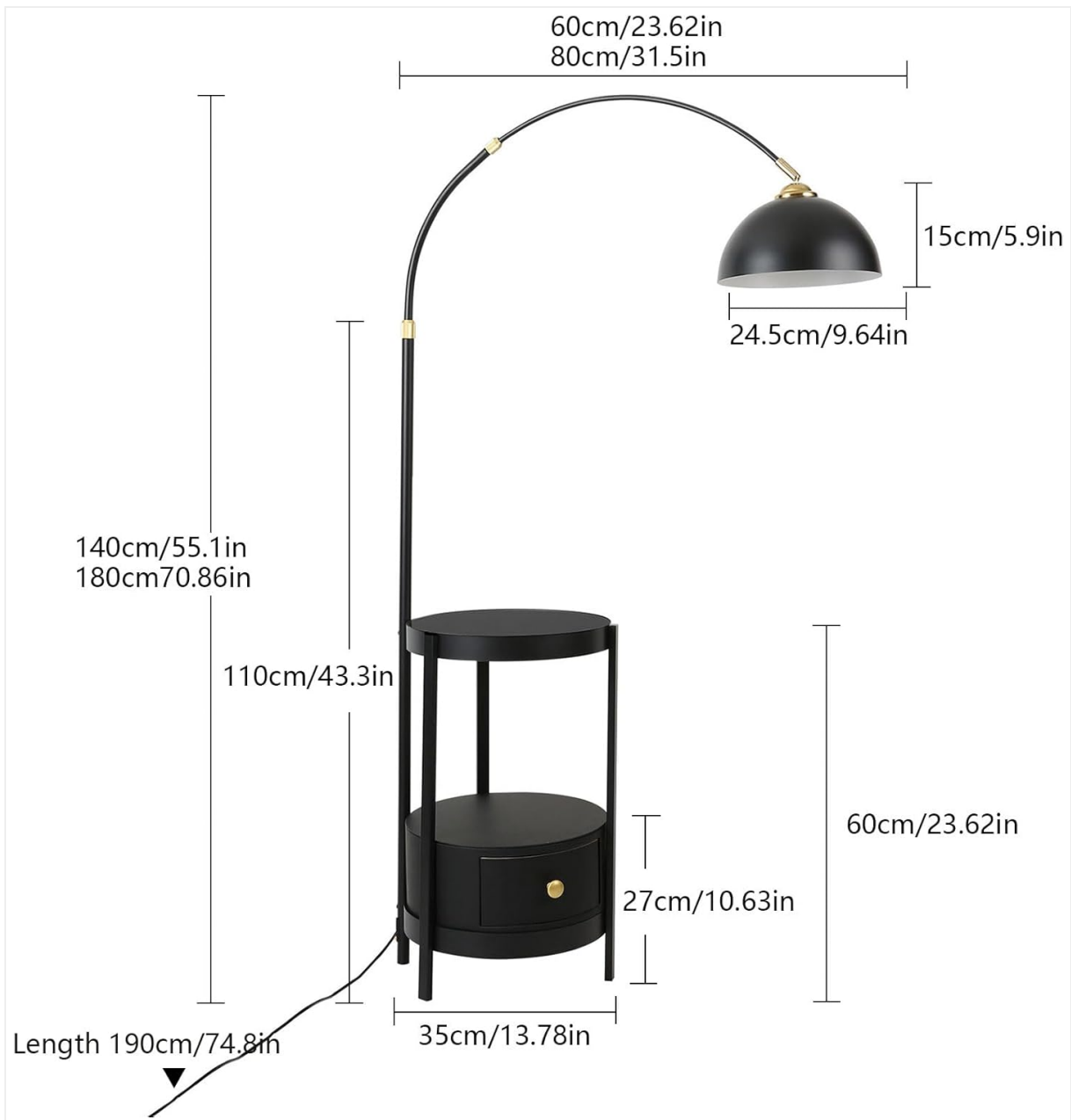
Image: A diagram illustrating the key dimensions of the floor lamp, including overall height, shade diameter, and base measurements.
