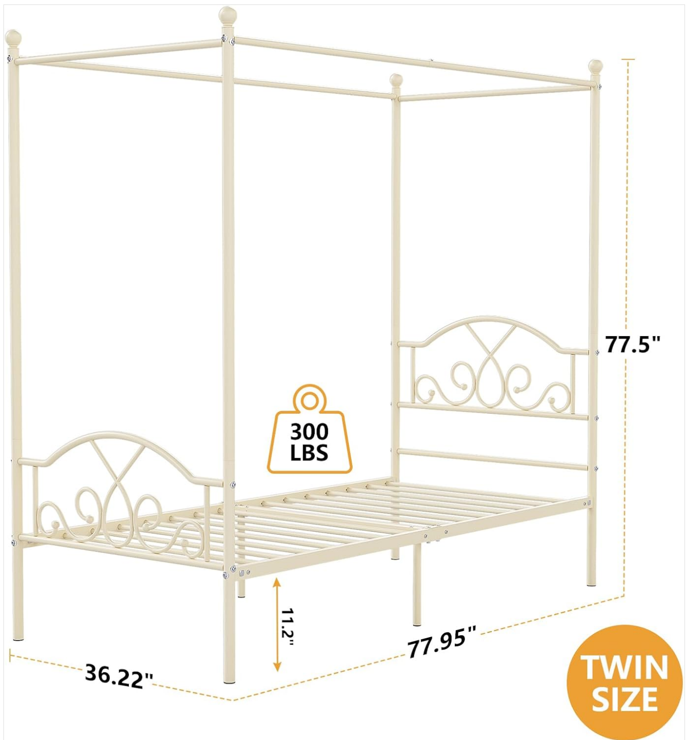
Figure 4.1: Key dimensions of the Twin Princess Canopy Bed Frame, including 11.2 inches of under-bed clearance.
