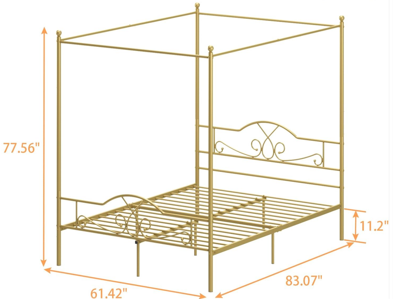
Figure 6: Detailed dimensions and weight capacity of the Queen size bed frame.
