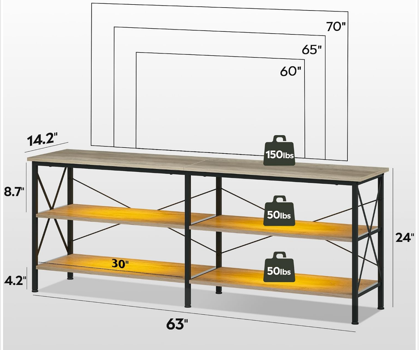
Image: Detailed product dimensions and maximum weight capacities for the desktop and shelves.
