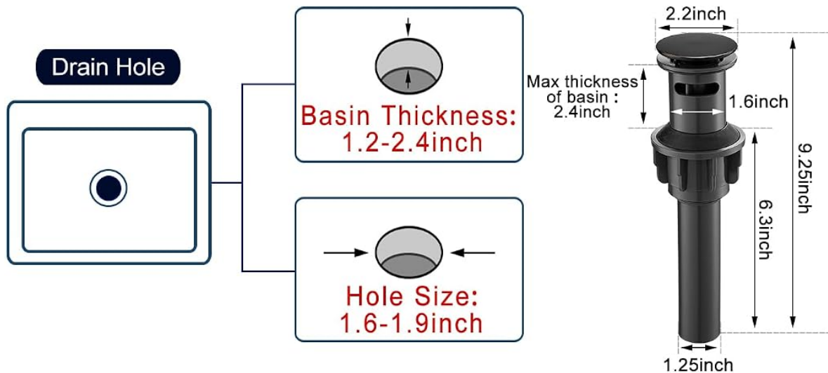
Figure 1: Overview of included faucet components.
