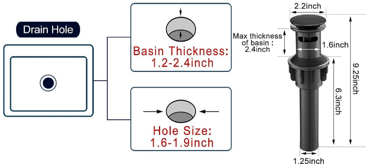
Figure 4: Pop-up drain installation guide and dimensions.
