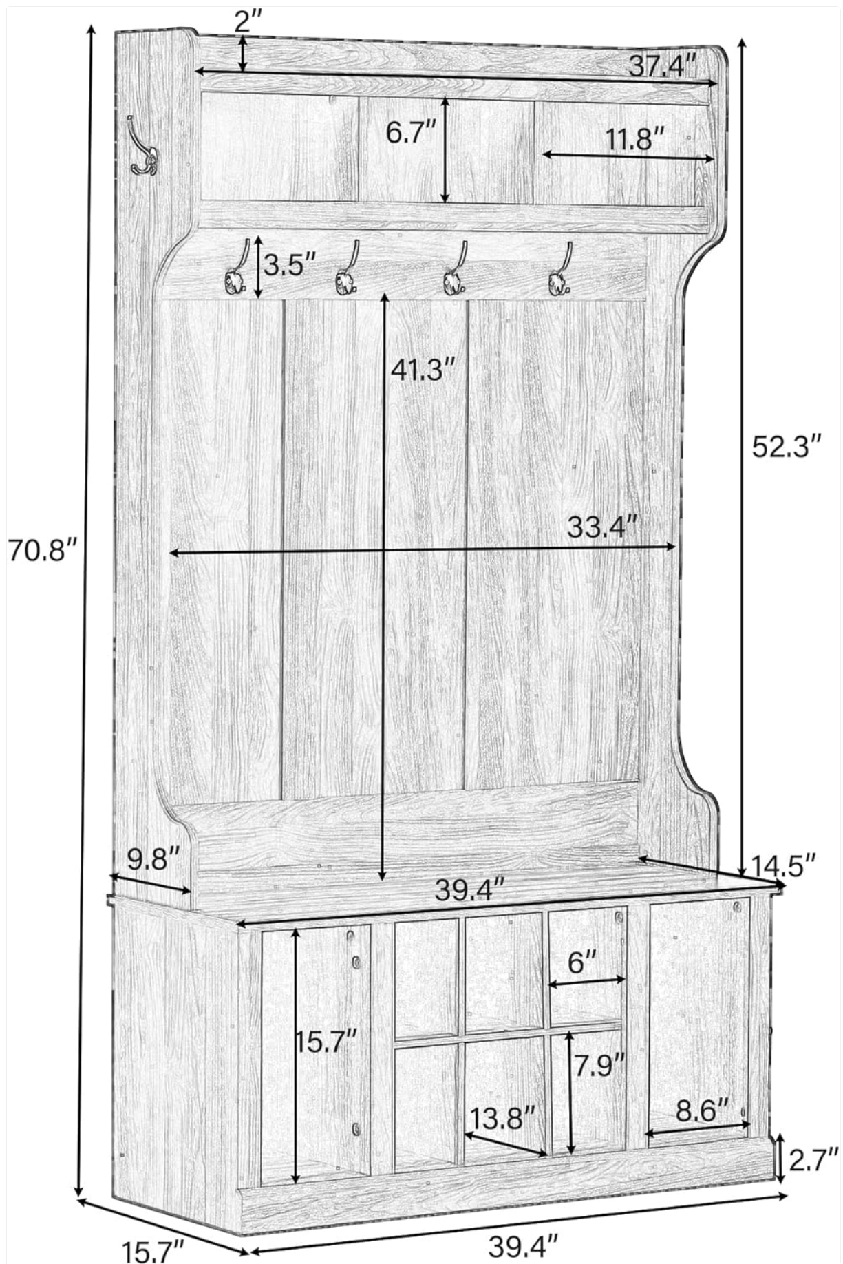
Image 4.1: Dimensional diagram of the Hall Tree, crucial for understanding component placement during assembly.
