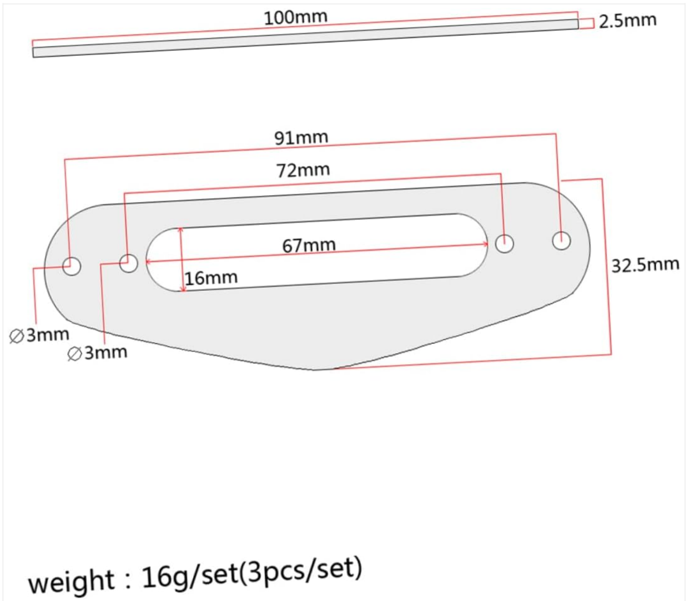
Image 2: Dimensional diagram of the VICASKY Gb405 mounting ring, showing key measurements for fitment.
