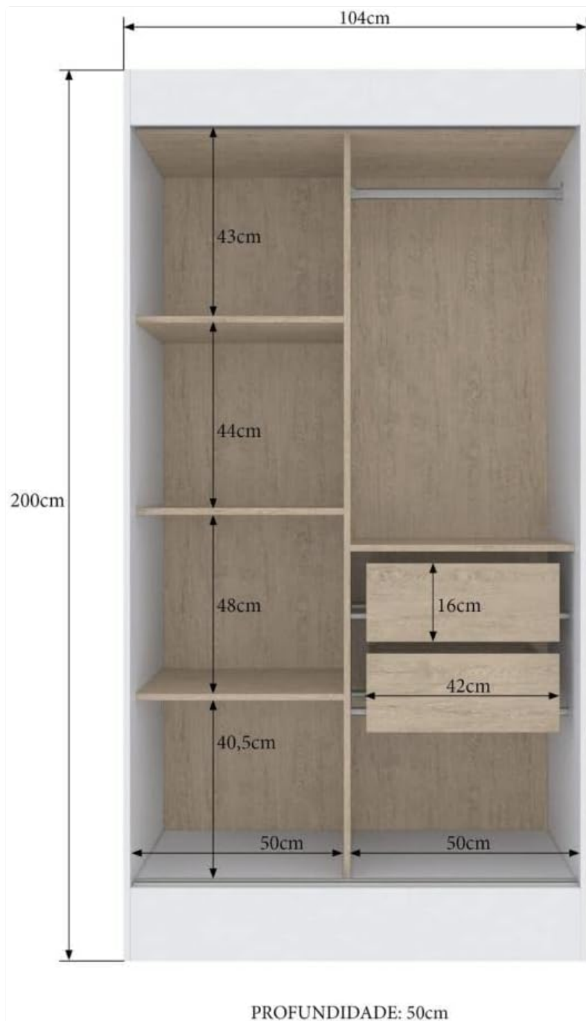
Figure 1: Front view of the Doripel Lyon Single Wardrobe, showcasing the two sliding doors with integrated mirrors.
